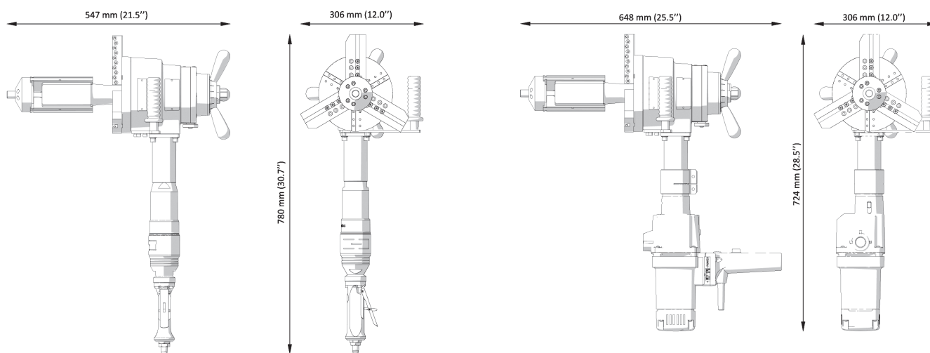
PRO-10 PB with pneumatic motor
